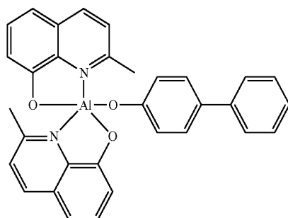
BAIq
